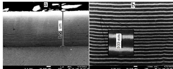
Fig. 2 – Cross-sectional SEM micrograph of TiN/MoN multilayer coating with 100 nm period: a – general view, thickness is 8.2 \mu\text{m} ; b – higher magnification (x 50 000) showing individual layer thickness.
